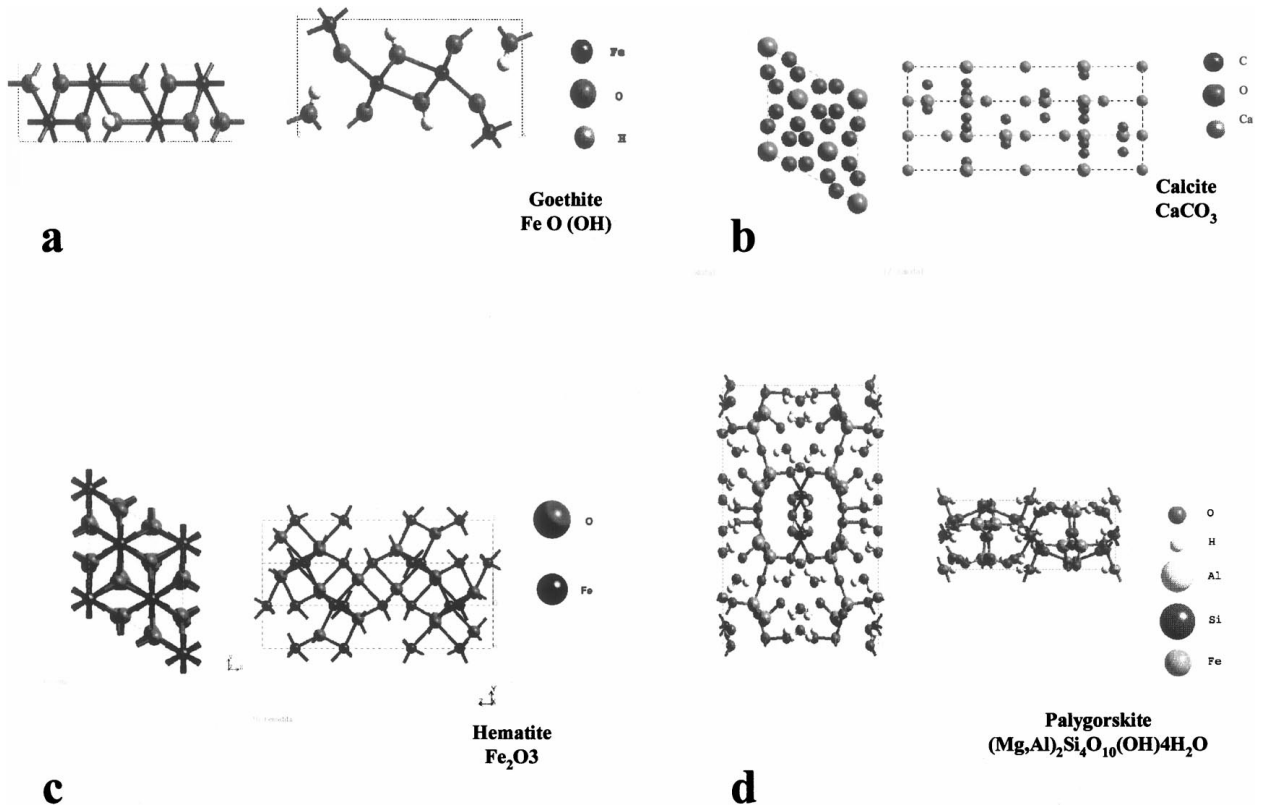
Figure 3 Unit cell view in two different orientations for each mineral found in pigments for the Aztec culture.
