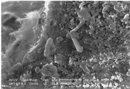
Figure 5 a) SEM secondary electron image showing the ochre color. Fibers and large crystals are observed that correspond to calcite and goethite mineral respectively. b) The expected crystal habit of calcite and c) the expected crystal habit of goethite.
