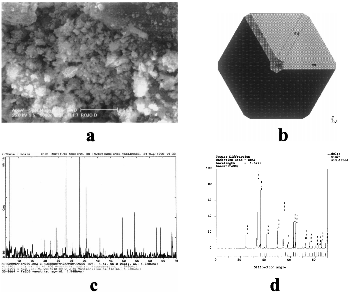
Figure 4 Results obtained for the red pigment which is composed by hematite ( \text{Fe}_2\text{O}_3 ). a) SEM secondary electron image showing the crystals. b) The expected habit for the hematite crystals. c) Experimental X-ray diffraction pattern of the red pigment. d) calculated X-ray diffraction pattern for hematite showing agreement with the one referred in c).
